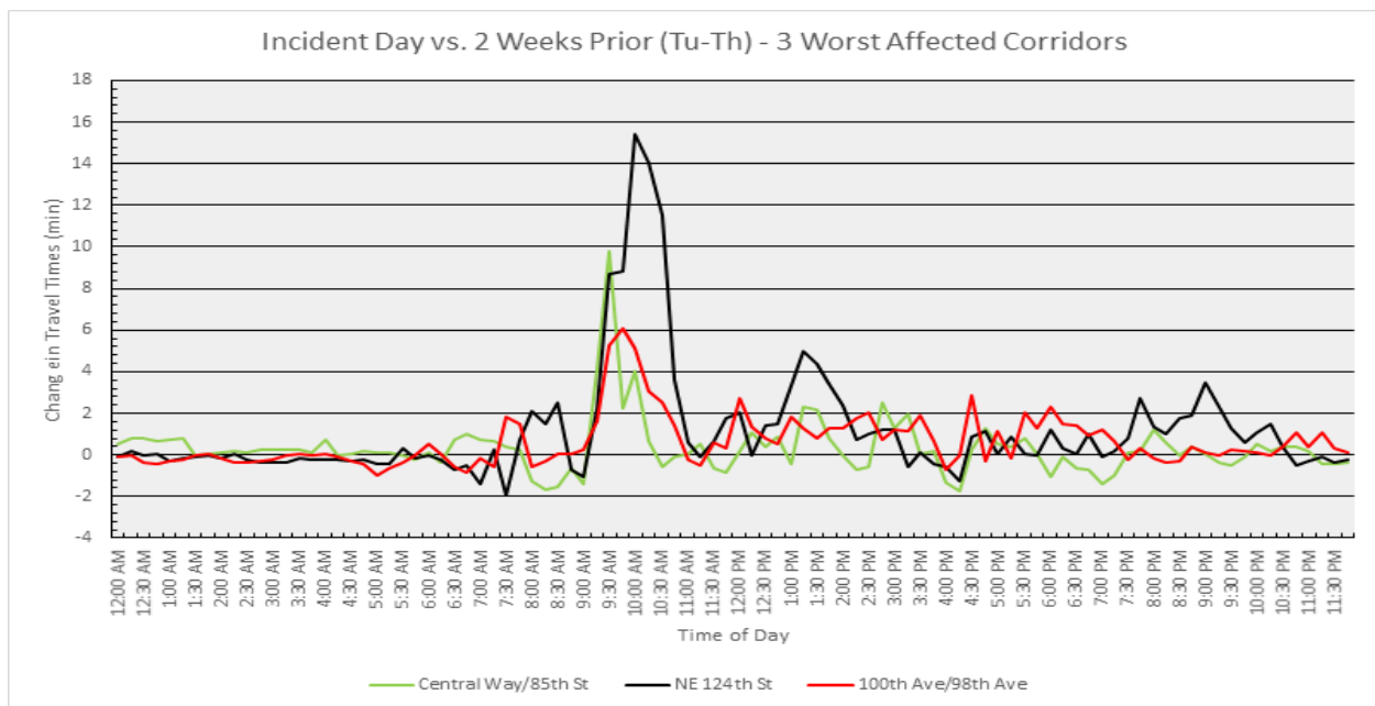
Figure 2-2: Change in Travel Time on Worst Affected Principal Arterials Due to October 10, 2018 Traffic Signal Flashing Operation
