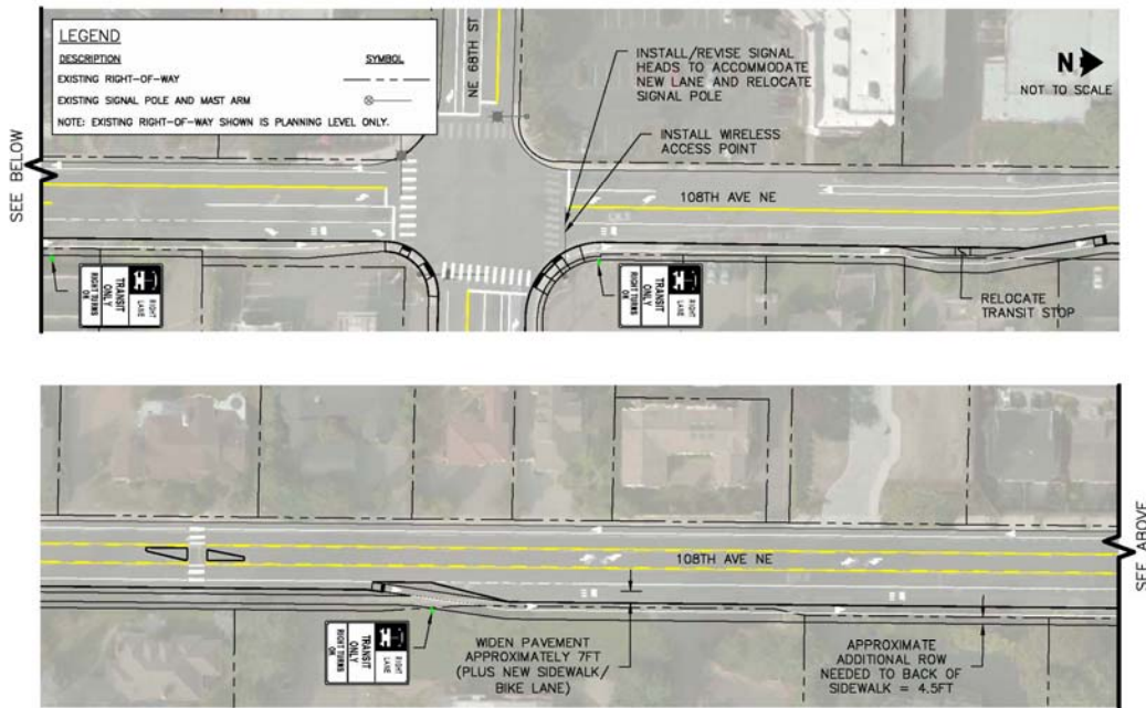
108th Ave NE and NE 68th St - Transit Signal Priority Improvement Concept F February 9, 2017 FIGURE 7F Kirkland 6th Street Corridor transpogroup 7F
