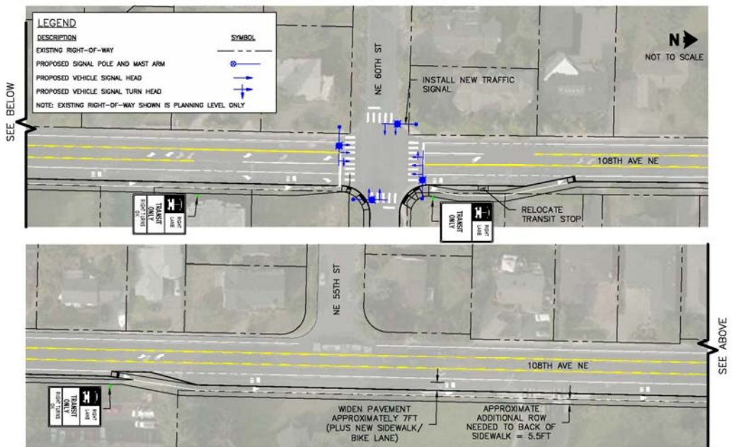
108th Ave NE and NE 60th St - Transit Signal Priority Improvement Concept E February 10, 2017 FIGURE 7E Kirkland 6th Street Corridor transpogroup 7E
